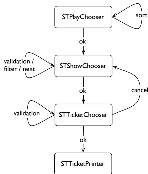
Figure 2: Theater-Flow as defined by STBuyTicketTask
